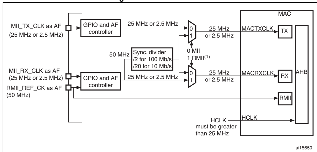
Figure 358. Clock scheme
