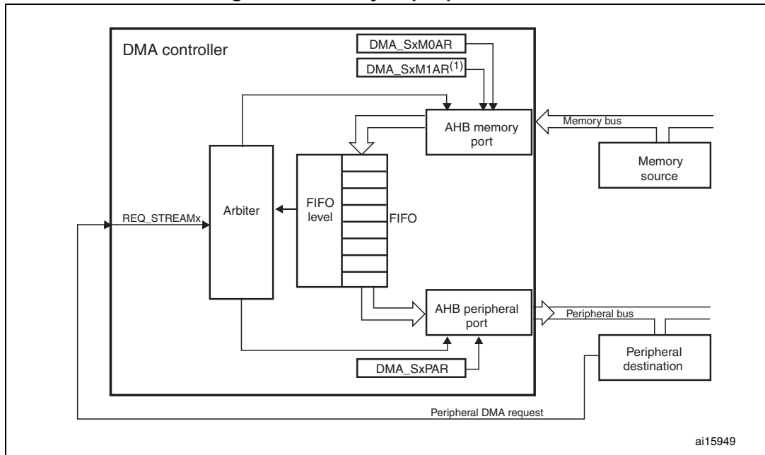
Figure 37. Memory-to-peripheral mode
