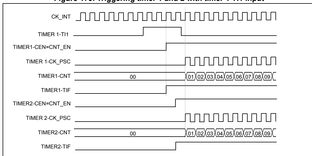
Figure 179. Triggering timer 1 and 2 with timer 1 T11 input
