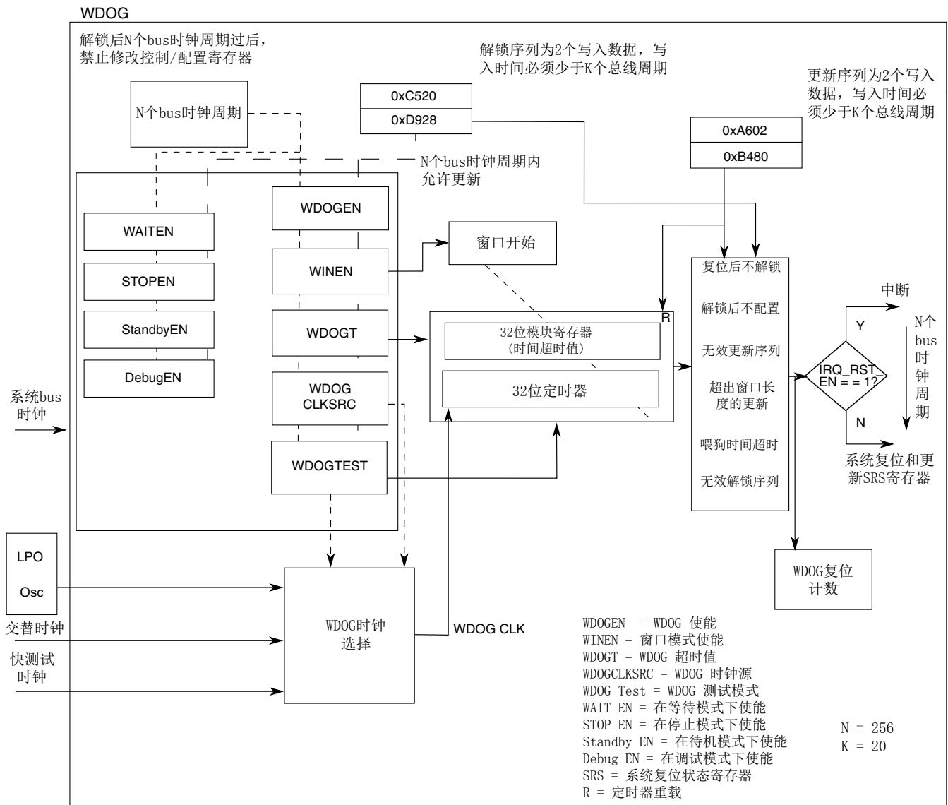
Figure 23-1. WDOG Operation
