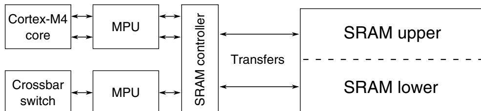
Figure 3-24. SRAM configuration
