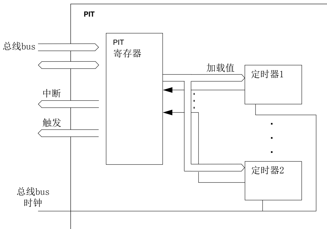
Figure 40-1. Block diagram of the PIT
